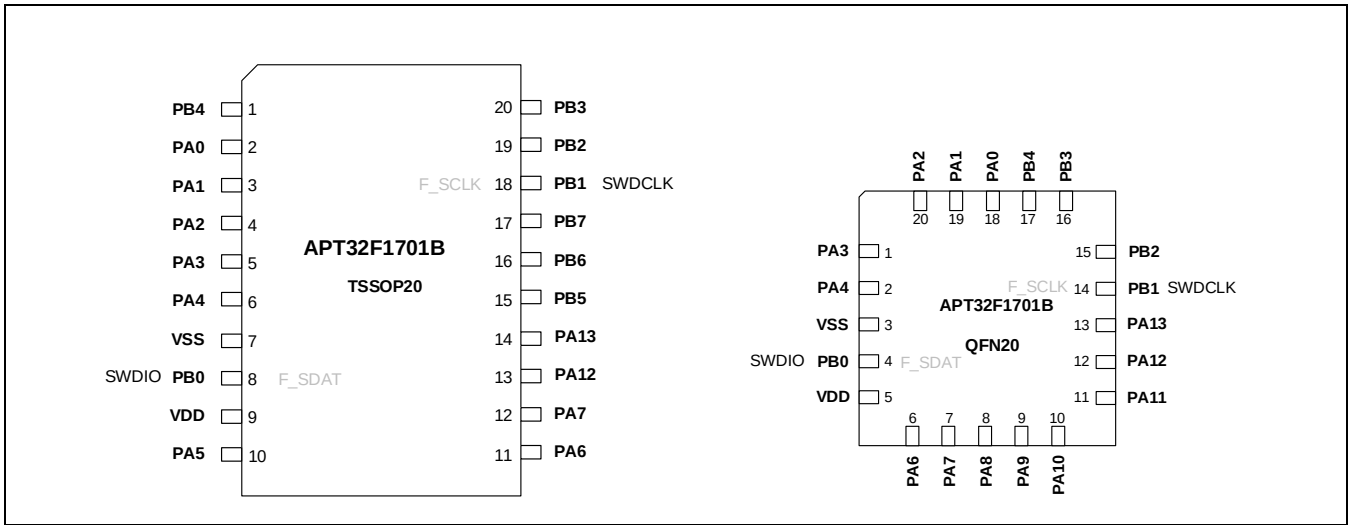
Figure 2-4 管脚定义图(TSSOP20, QFN20)
