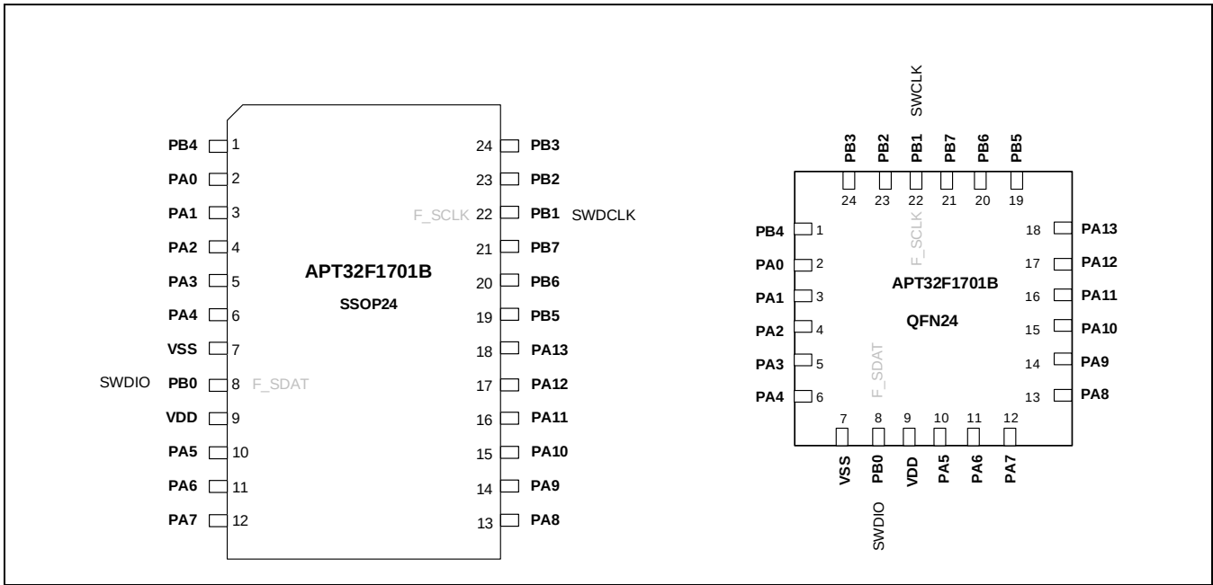
Figure 2-3 管脚定义图(SSOP24, QFN24)
