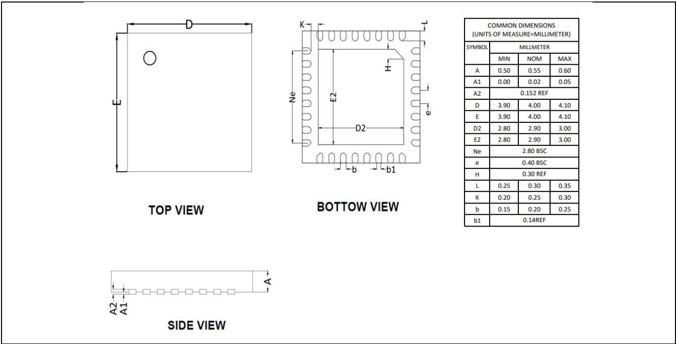
Figure 4-2 QFN32 (P0.4mm)封装尺寸
