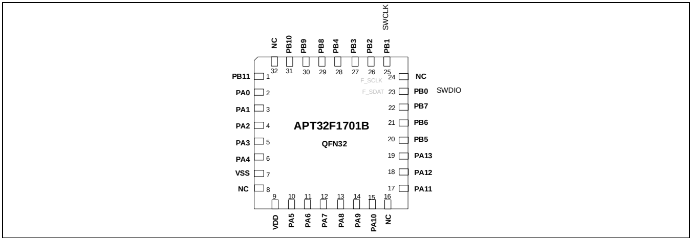
Figure 2-1 管脚定义图(QFN32)
