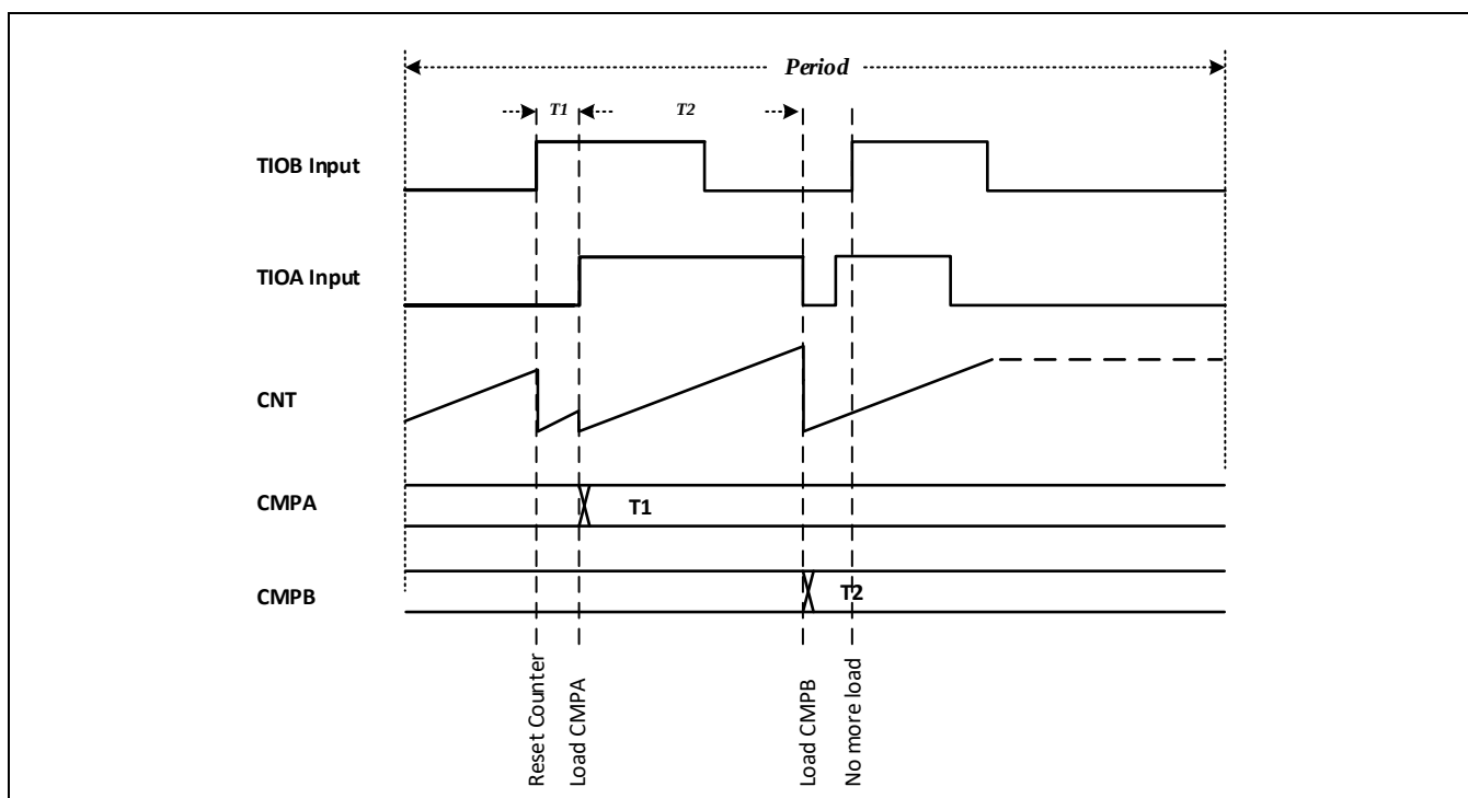
Figure 13-13 测量TIOA和TIOB相位差
