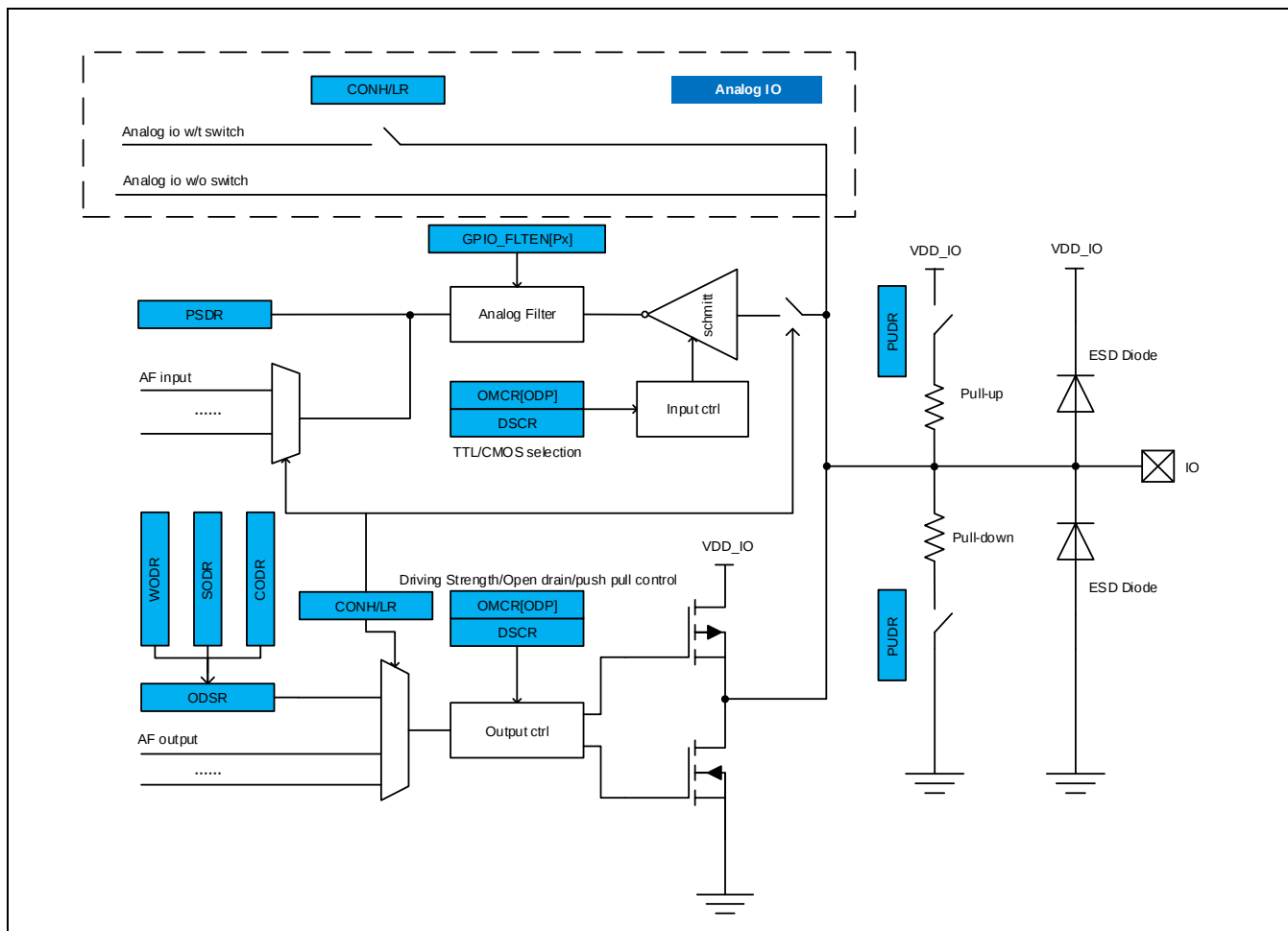
Figure 7-1 GPIO原理图
