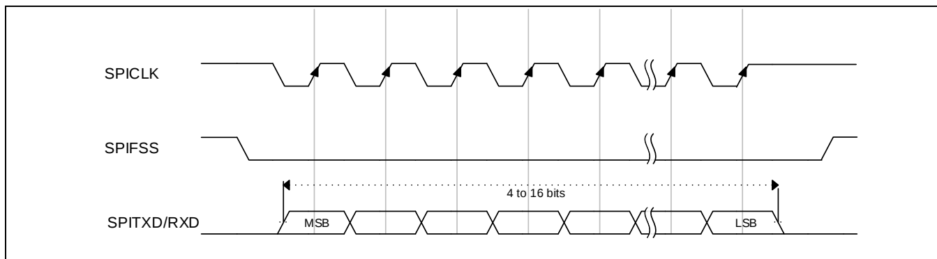
Figure 16-11 Motorola SPI 帧格式(单帧传输), SPO = 1 和 SPH = 1
