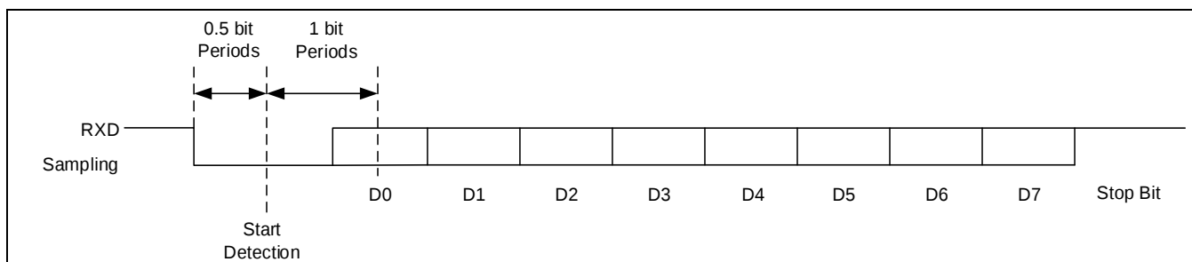
Figure 15-3 接收数据
