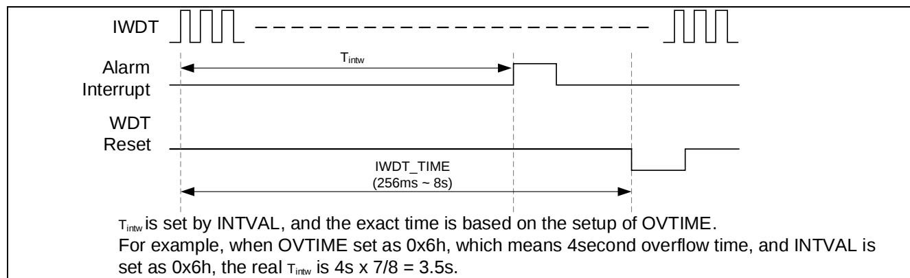
Figure 5-10 IWDT 计数器溢出和报警中断
