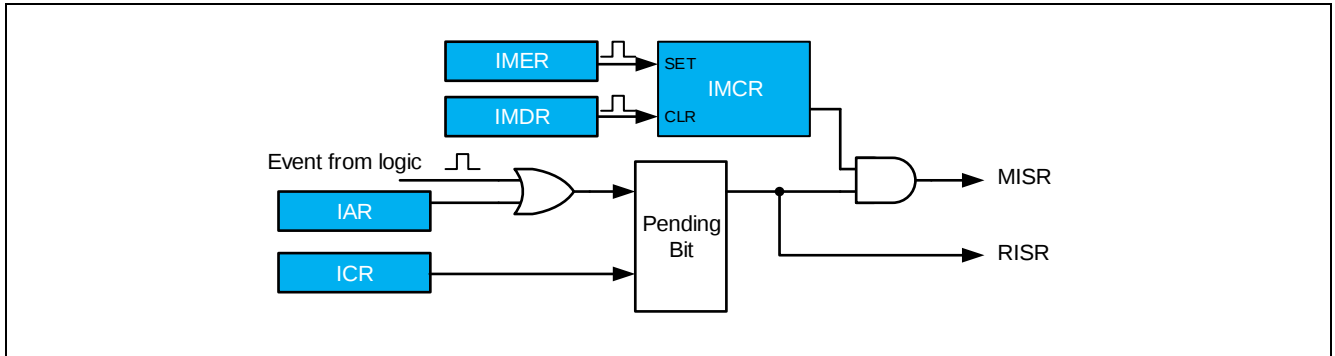
Figure 5-11 SYSCON 通用中断的控制逻辑
