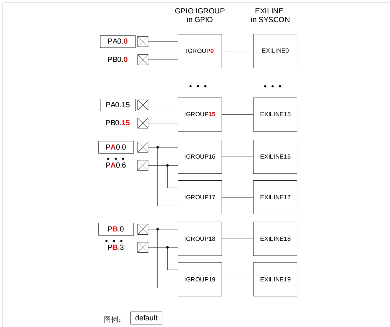
Figure 7-2 GPIO IGROUP和 SYSCON中的EXILINE
