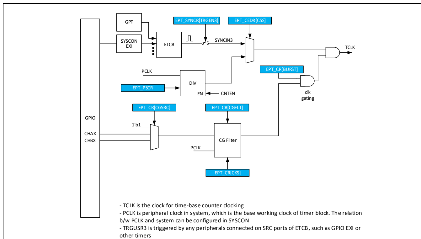
Figure 14-2 时钟控制模块
