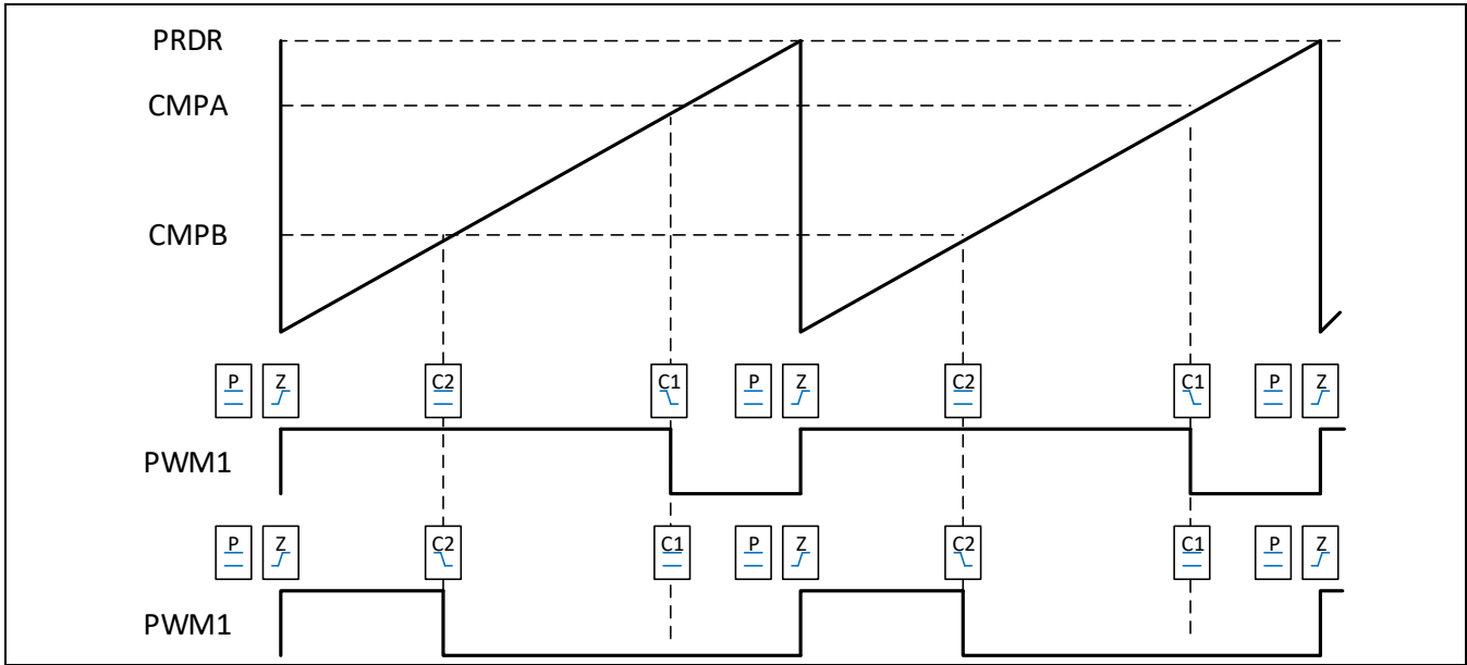
Figure 13-11 递增单沿，非对称波形输出
