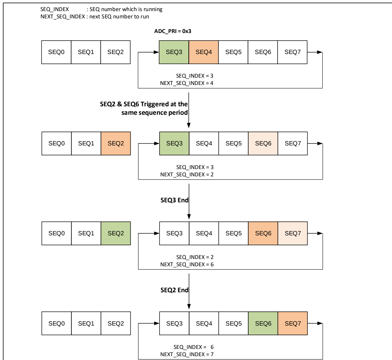
Figure 9-8 触发优先级示意图
