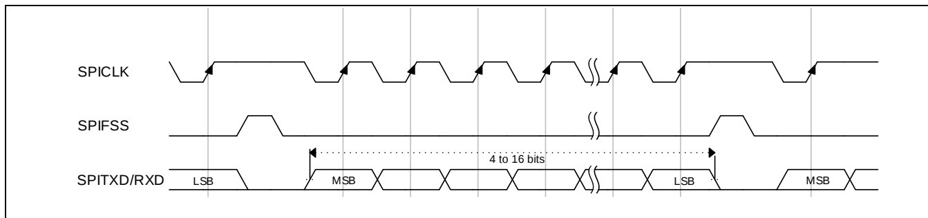
Figure 16-12 Motorola SPI 帧格式(连续传输), SPO = 1 和 SPH = 1
