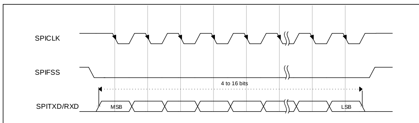
Figure 16-10 Motorola SPI 帧格式 (连续传输), SPO = 1 和 SPH = 0
