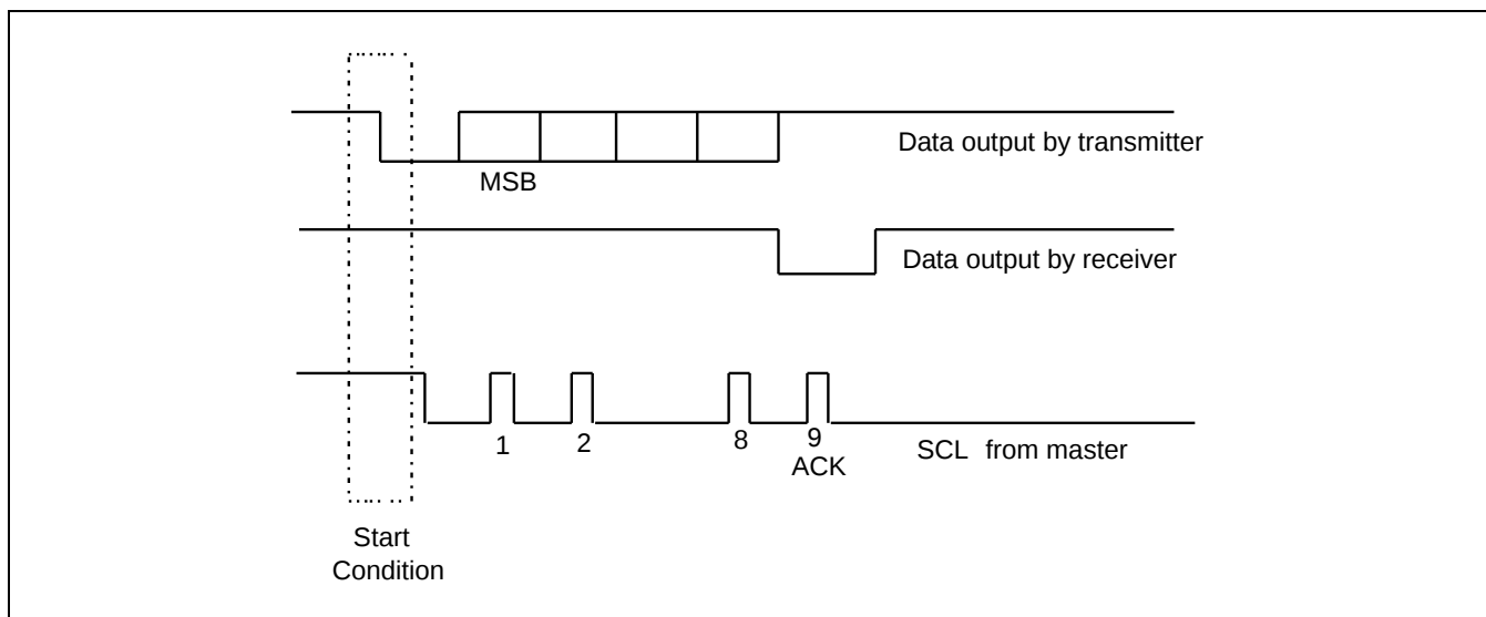
Figure 17-5 应答
