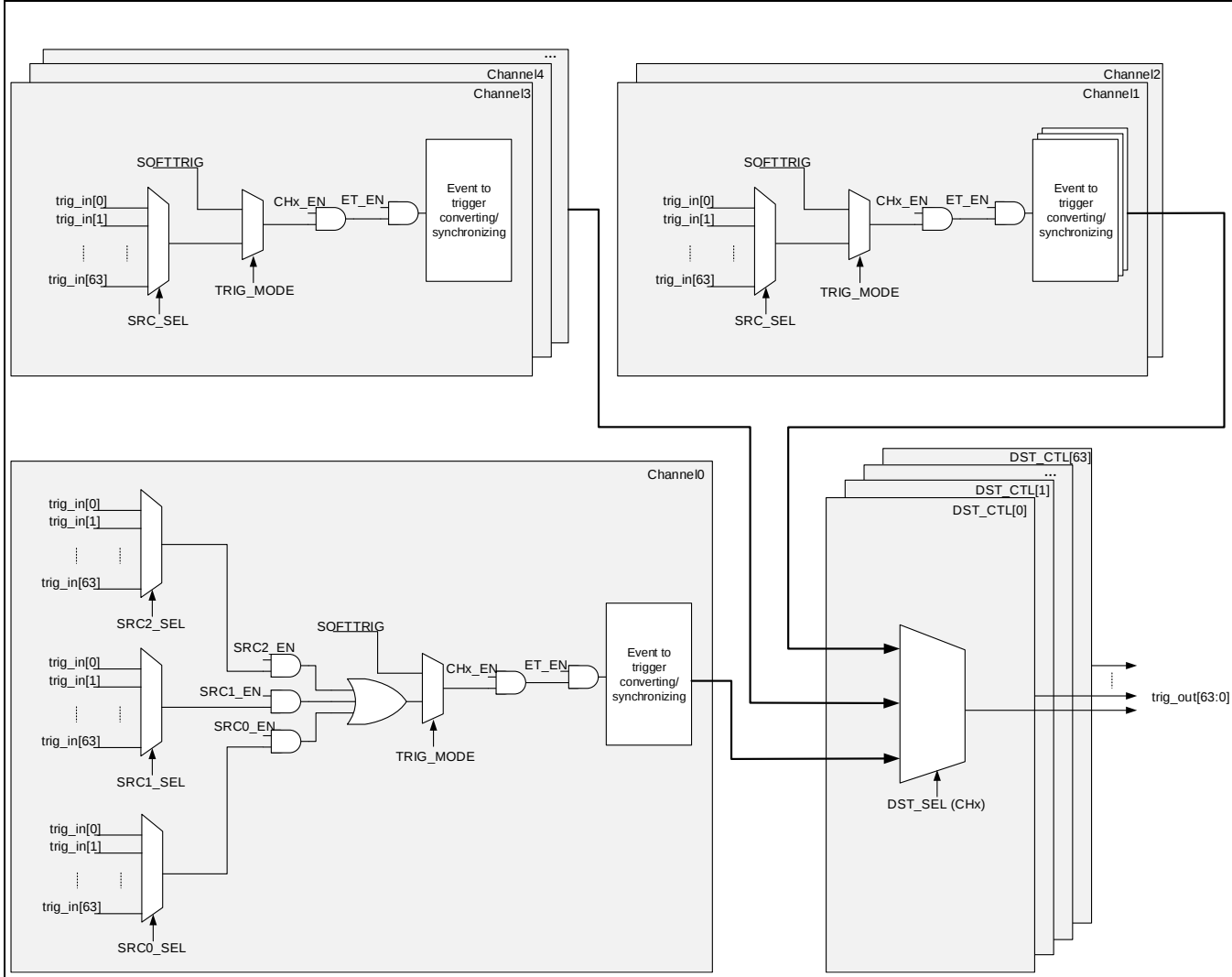
Figure 8-1 ETCB模块框图
