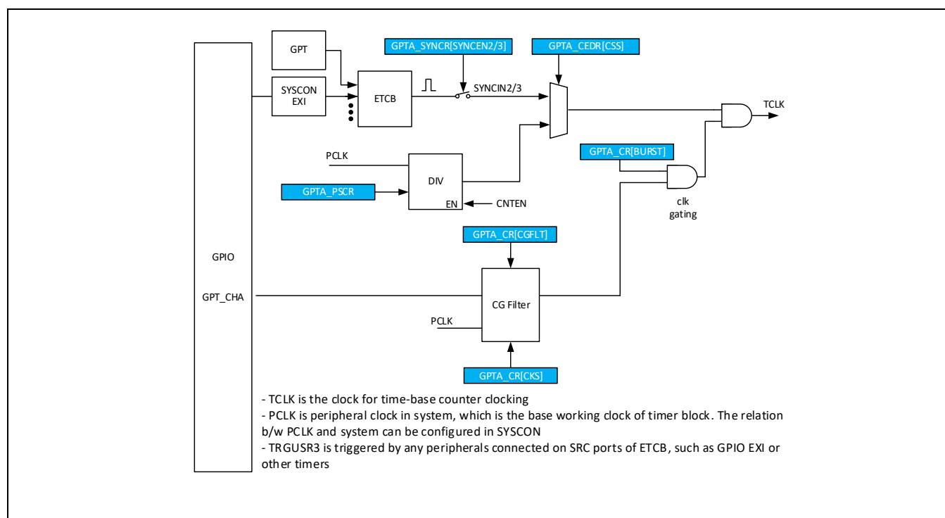
Figure 13-2 时钟控制模块
