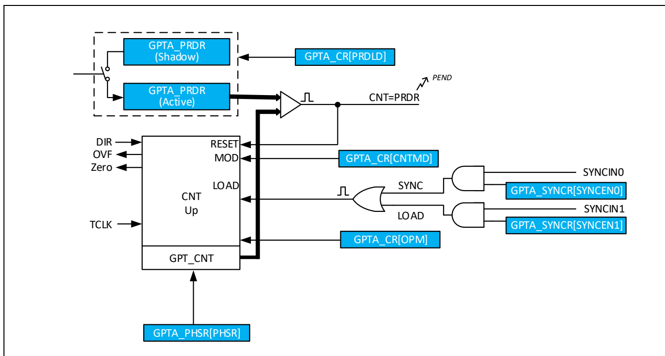
Figure 13-5 计数器时基模块
