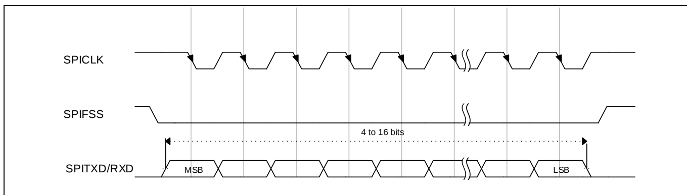
Figure 16-9 Motorola SPI 帧格式 (单帧传输), SPO = 1 和 SPH = 0
