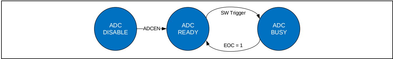
Figure 9-3 ADC状态机
