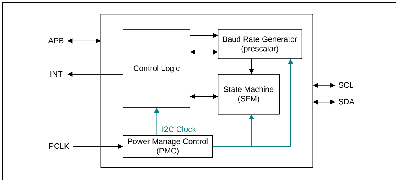
Figure 17-1 I2C模块框图
