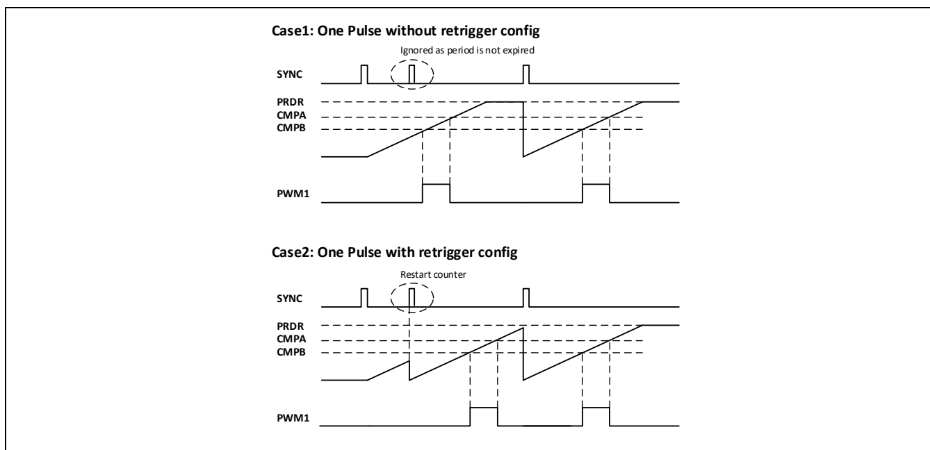
Figure 14-36 单次触发
