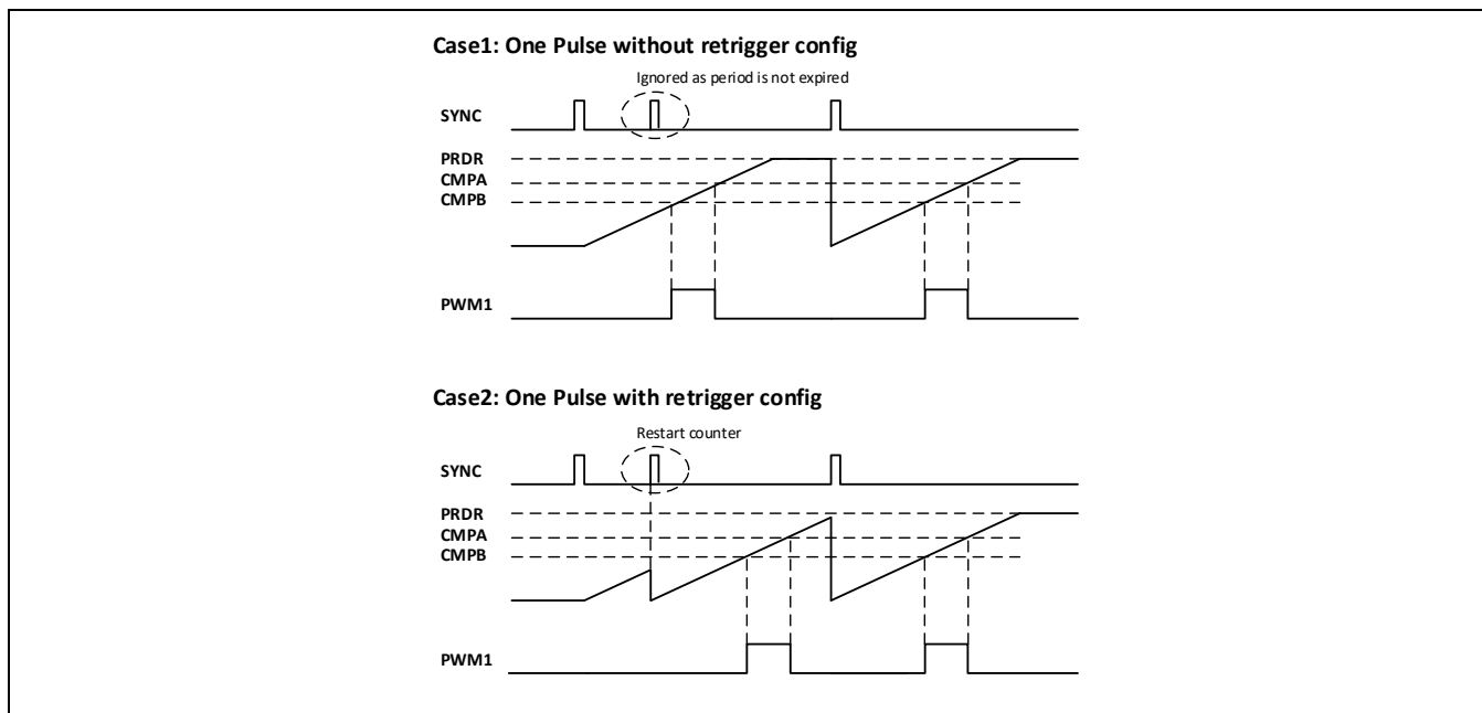
Figure 13-15 单次触发
