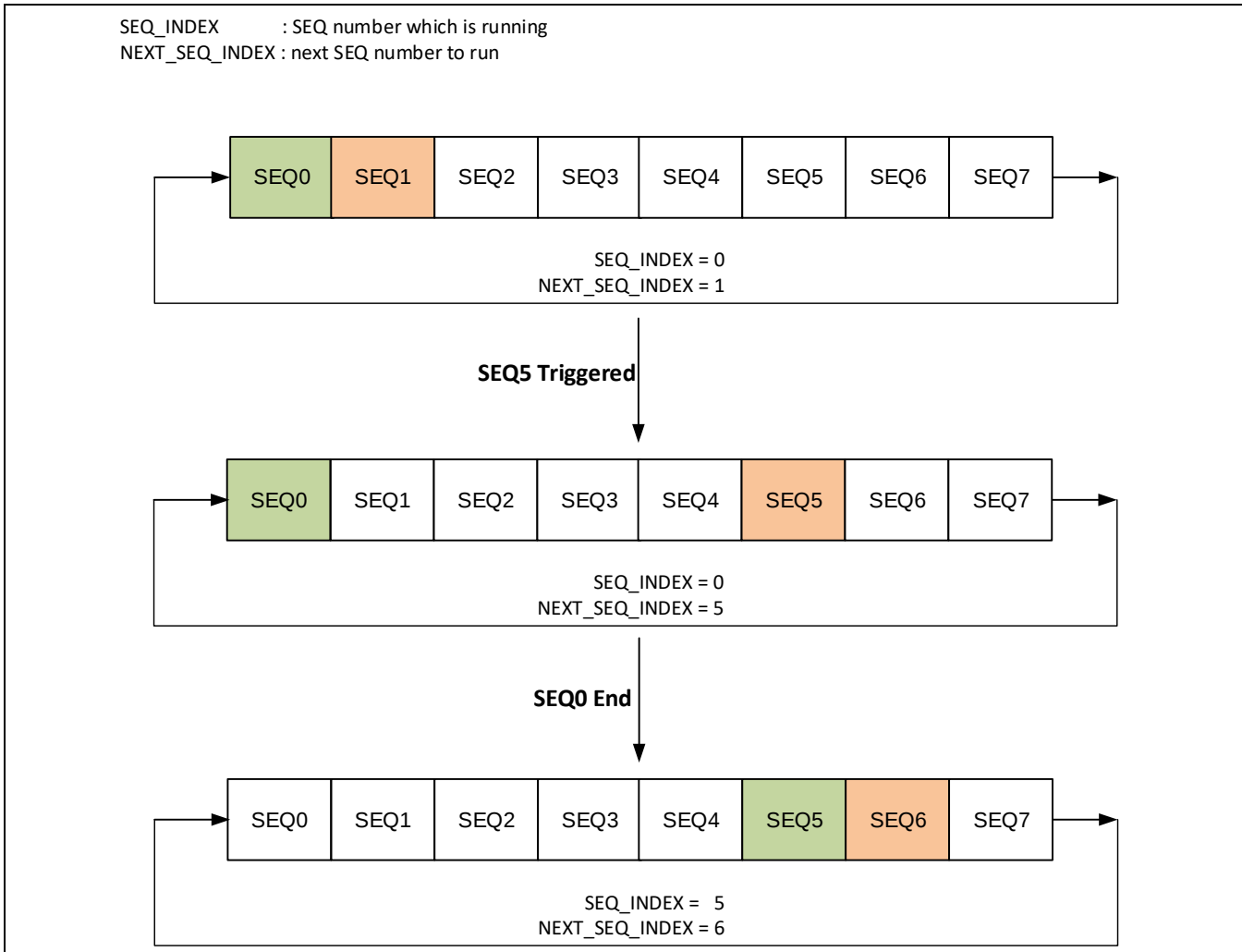
Figure 9-6 触发原理示意图
