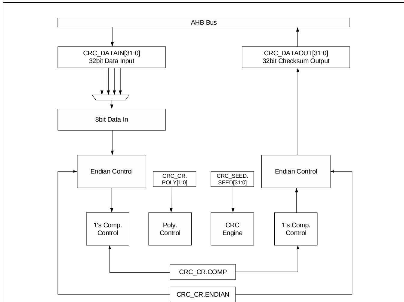
Figure 6-1 CRC模块框图
