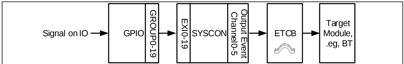
Figure 5-12 Signal Flow
