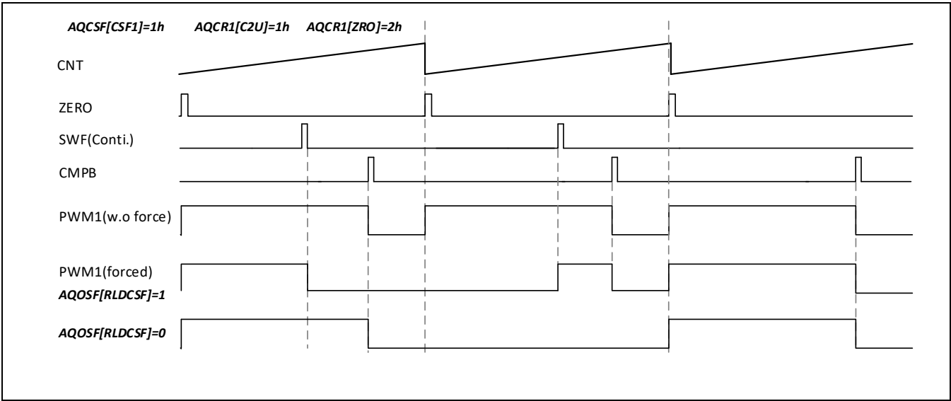
Figure 14-21 持续性软件强制输出
