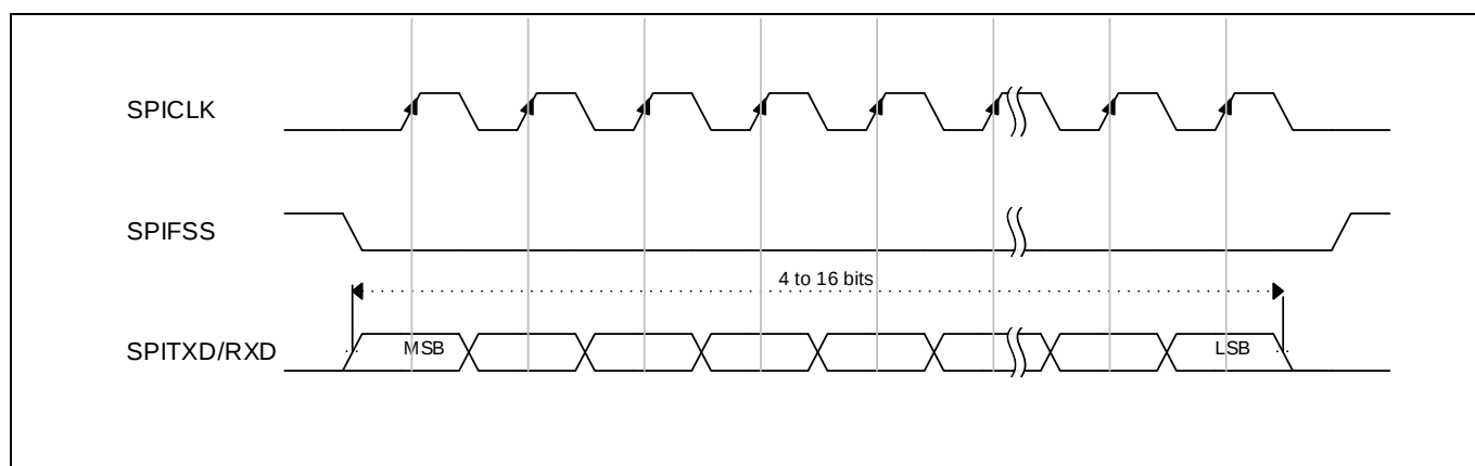
Figure 16-5 Motorola SPI 帧格式 (单帧传输) SPO = 0, SPH = 0
