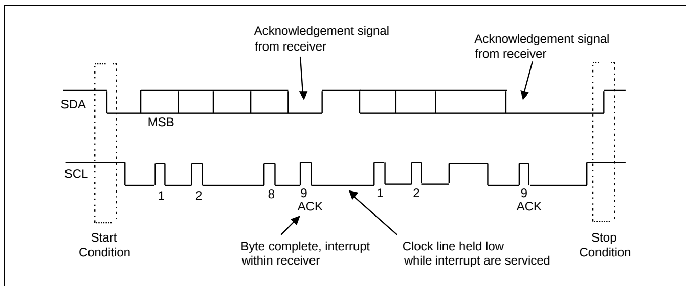
Figure 17-4 I2C总线的数据传输
