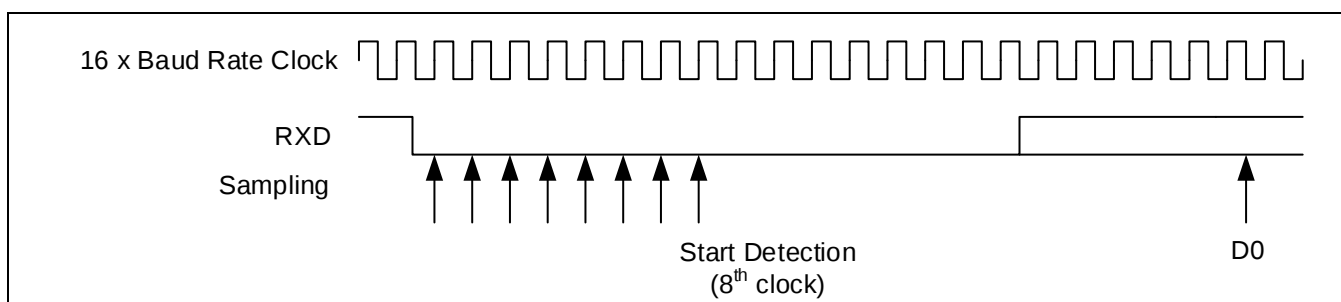
Figure 15-2 起始位检测
