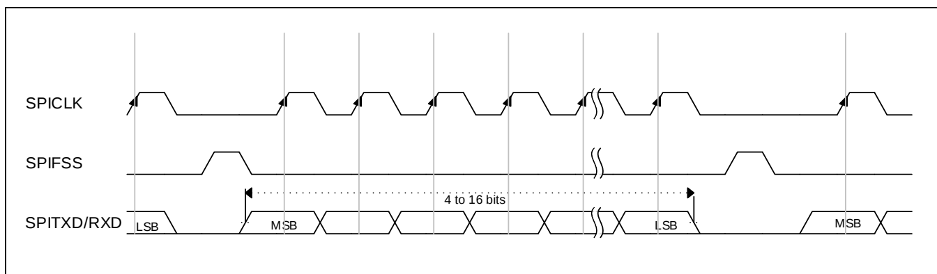
Figure 16-6 Motorola SPI 帧格式 (连续传输) SPO = 0, SPH = 0
