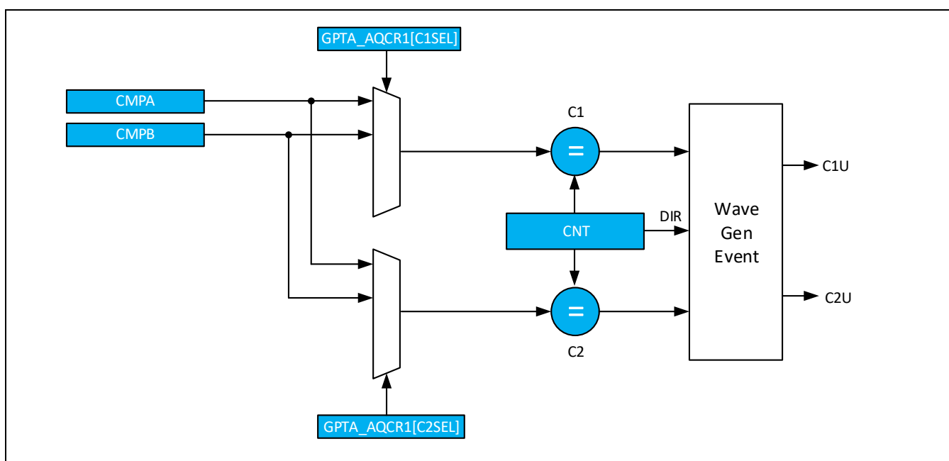
Figure 13-10 C1 and C2 selection control
