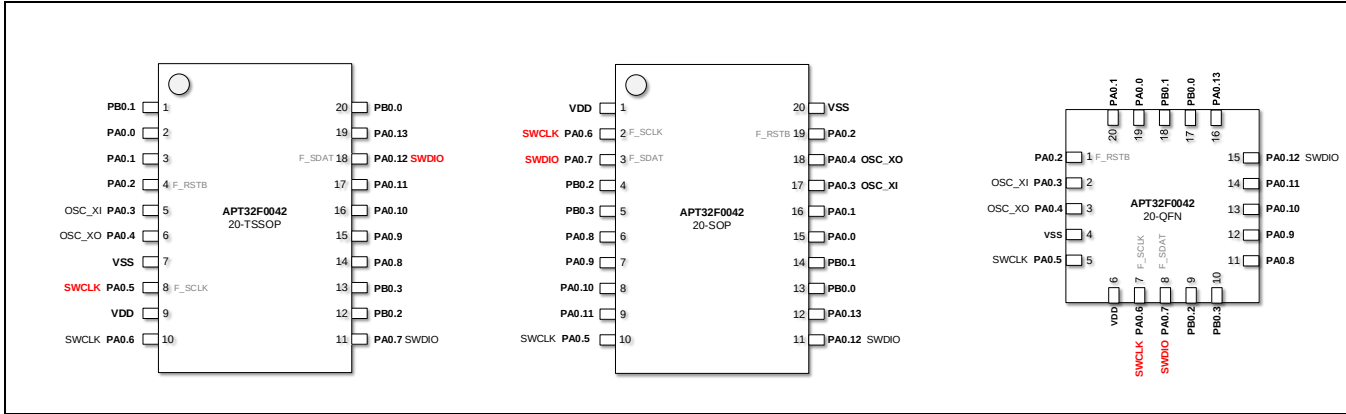
Figure 2-1 管脚定义图(TSSOP20, SOP20, QFN20)
